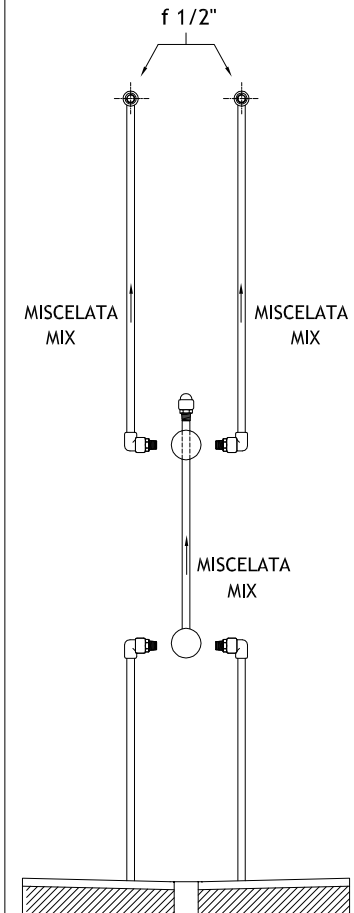
SCHEMA IDRAULICO PLUMBING CONNECTION
