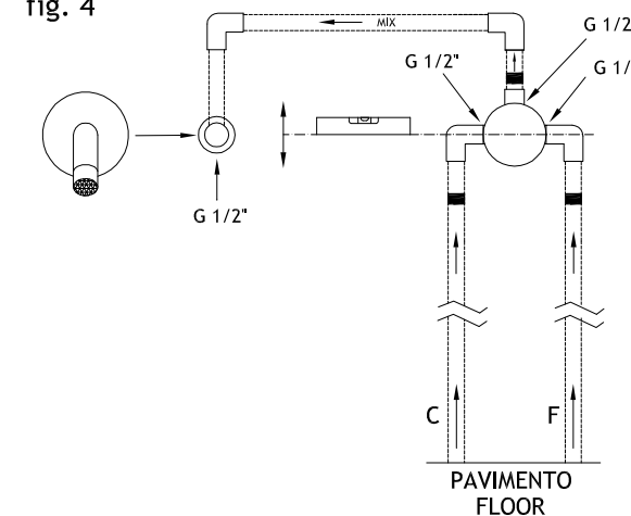
SCHEMA IDRAULICO PLUMBING CONNECTIONS
