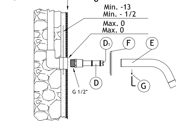
SCHEMA IDRAULICO PLUMBING CONNECTIONS
